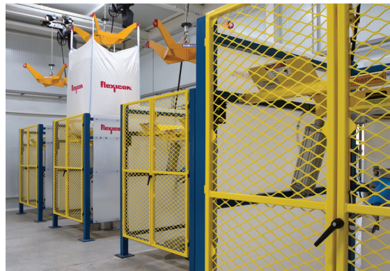
Seven Bulk-Out® model BFC-C-X half-frame bulk bag dischargers feed 70 tonnes per day to packaging machines on the floor below. An electric hoist positioned over each discharger lifts the bag onto the half frame.
