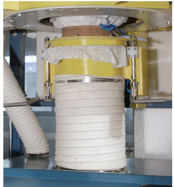
At the bag spout interface, a SPOUT-LOCK clamp ring creates a dust-tight seal while a TELE-TUBE telescoping tube maintains constant downward pressure as the bag empties/elongates, promoting complete discharge.
