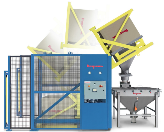
The light curtain feature on this new TIP-TITE® Container Dumper from Flexicon allows a single operator to load and unload containers without leaving the fork truck. The device automatically stops the machine if someone enters the hazard zone.
